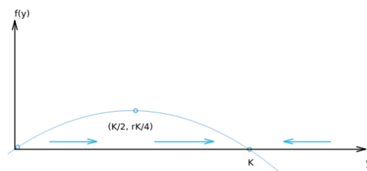
Figure 5.14: The equilibrium solution f(y) = 0 or r(1 - y/K)y = 0 to visualize other solutions of Eq. (4.53) ( Hamzstplot/Examples with Makefile/Plot 2D Equilibrium Solution for Logistic Growth/main.cpp ).
