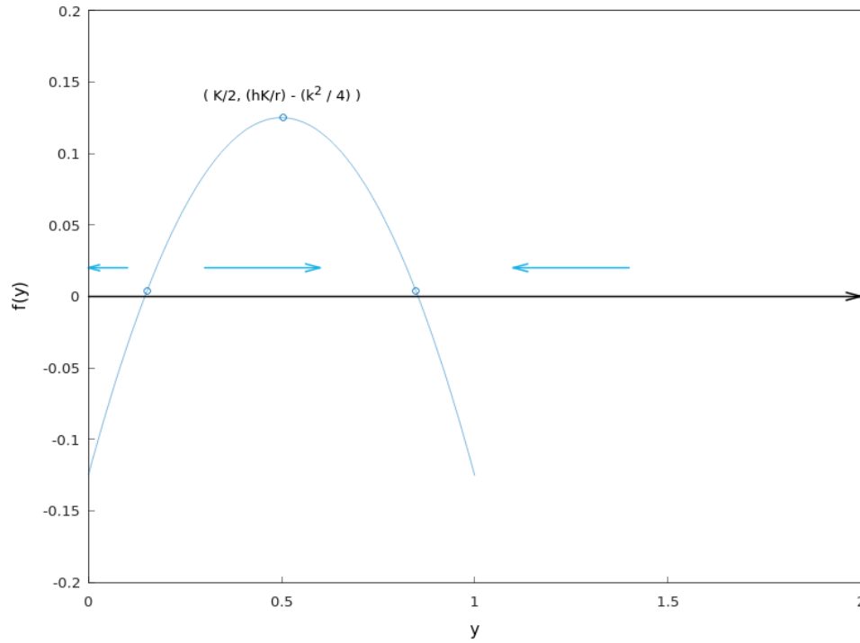
Figure 5.23: The plot for f(y) = (1 - y)y - \frac{1}{8} (Hamzstplot/Examples with Makefile/Plot 2D Equilibrium Solution for Schaefer Model Variation/main.cpp).
