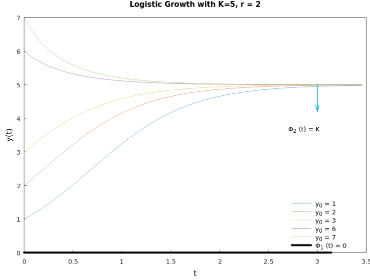
Figure 5.15: The solution curves for y(t) = \frac{y_0 K}{y_0 + (K - y_0)e^{-rt}} to visualize all possible solutions of Eq. (4.53) with different y_0 (Hamzstplot/Examples with Makefile/Plot 2D Solution Curves for Logistic Growth/main.cpp).
