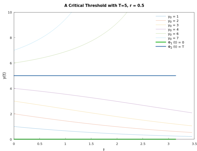
Figure 5.18: The solution curves for growth with a threshold for \frac{dy}{dt} = -r \left(1 - \frac{y}{T}\right) y (Hamzstplot/Examples with Makefile/Plot 2D Solution Curves for Critical Threshold/main.cpp).
