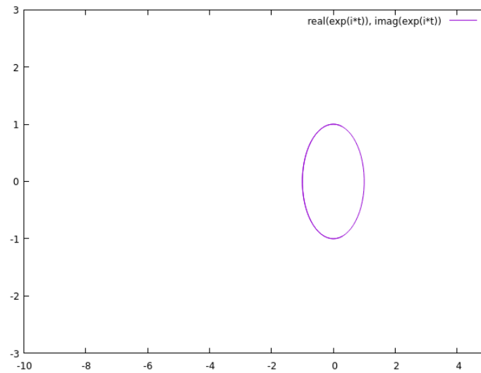
Figure 12.4: The 2D parametric plot of (\text{real}(e^{ix}), \text{imag}(e^{ix})) (DFSimulatorC/Source Codes/C++/C++ Gnuplot SymbolicC++/ch23-Numerical Linear Algebra/2D Plot Complex Function/main.cpp).
